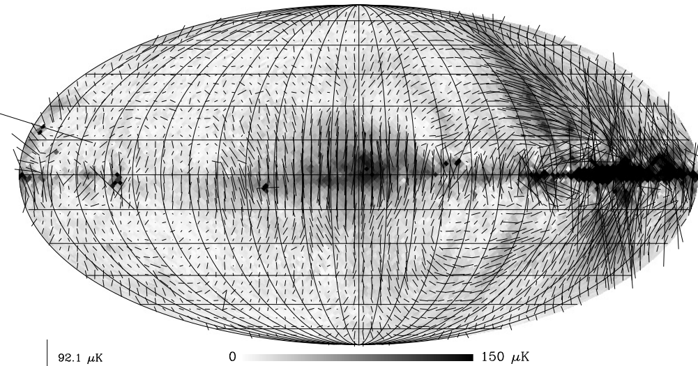
23 GHz polarized intensity (WMAP)
