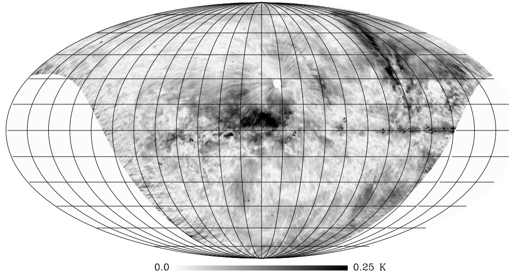
23 GHz polarized intensity (WMAP)
