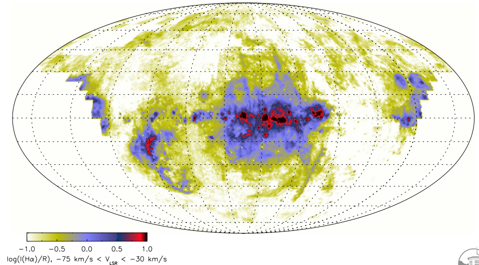
H \alpha intensity (WHAM)
